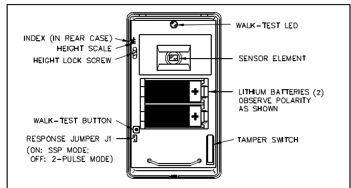
GEM-PIR, front cover removed.
